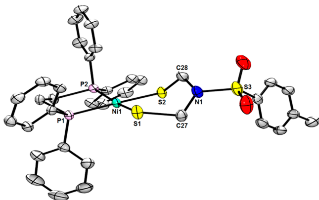
Figure 6. ORTEP of Ni[(SCH 2 ) 2 NTs](dppe) with ellipsoids drawn at the 50% probability level. H atoms and disorder are omitted for clarity. Selected distances (Å): Ni1–S1, 2.1943(5); Ni1–S2, 2.1963(5); Ni1–P1, 2.1804(5); Ni1–P2, 2.1873(5). Selected angles (deg): S1–Ni1–S2, 94.568(19); P1–Ni1–P2, 87.143(18); P1–Ni1–S1, 90.505(18); P2–Ni1–S1, 168.68(2); P1–Ni1–S2, 173.82(2); P2–Ni1–S2, 88.549(18); C27–N1–C28, 116.95(15), C27–N1–S3, 119.69(13); C28–N1–S3, 117.26(13).
